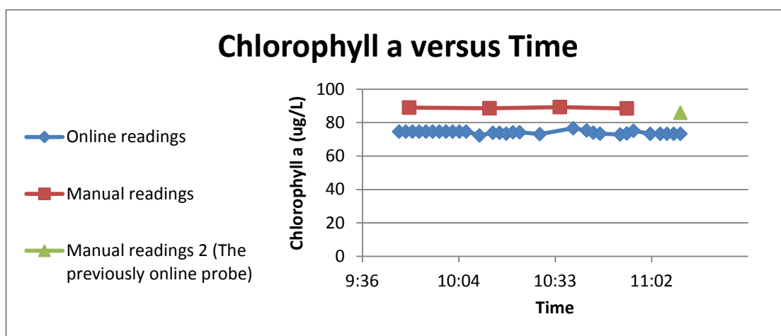
Figure 53 Chlorophyll concentration change over time in Pitkajärvi, online and manual readings
