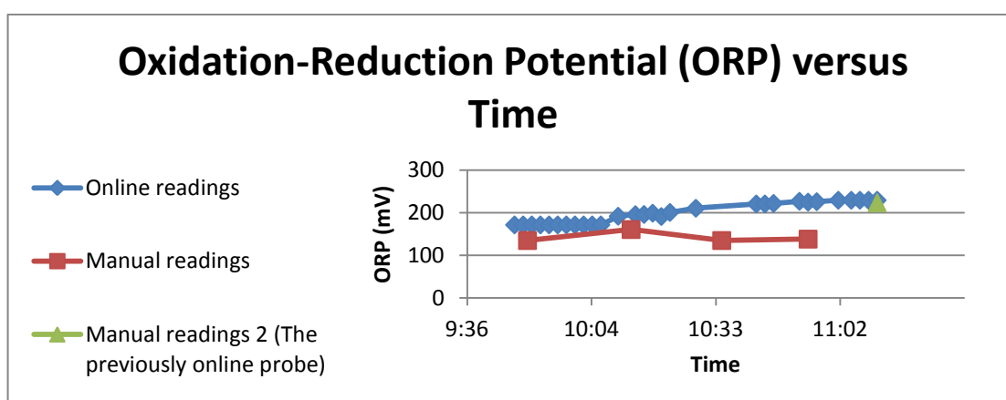
Figure 59 ORP change over time in Pitkäljärvi, online and manual readings
