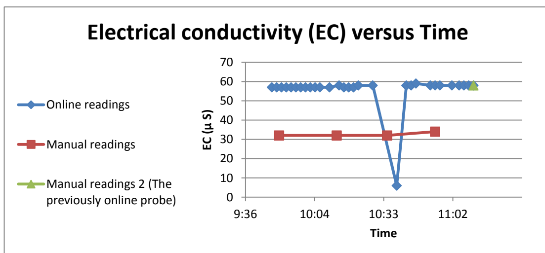
Figure 45 the EC change over time in Pitkäjärvi, online and manual readings
