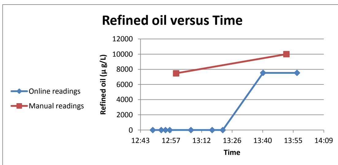
Figure 64 Refined oil change over time in Tuppurala, online and manual readings
