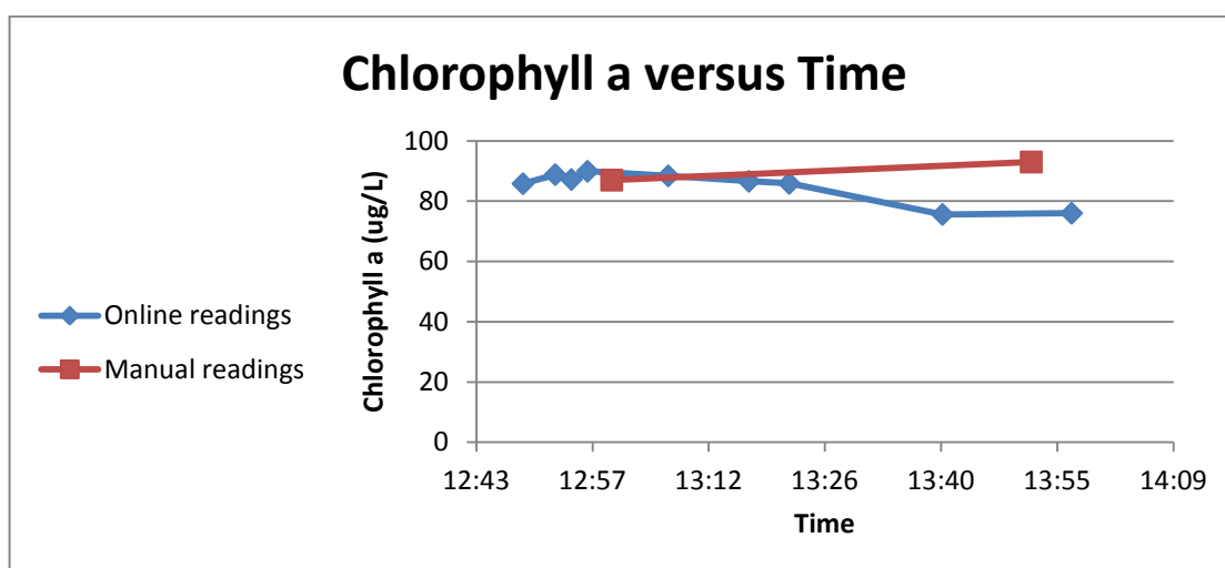
Figure 52 Chlorophyll concentration change over time in Tuppurala, online and manual readings
