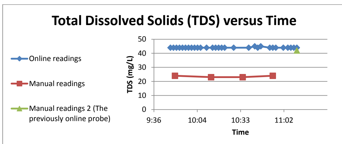
Figure 49 TDS change over time in Pitkäjärvi, online and manual readings
