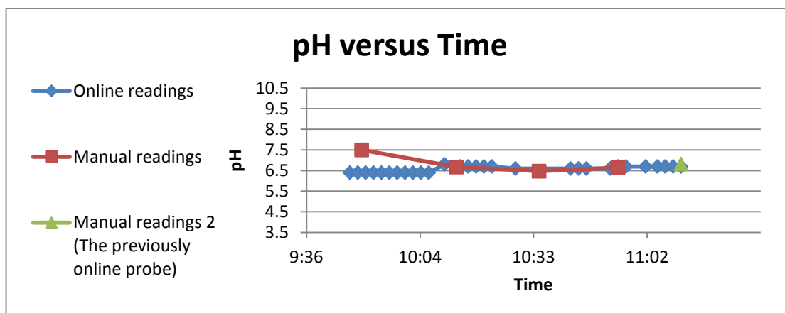
Figure 40 The pH change over time in Tuppurala, online and manual readings
