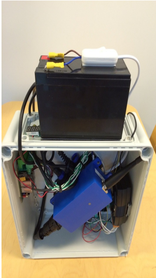
Figure 11 The main component of the PaquaBag
