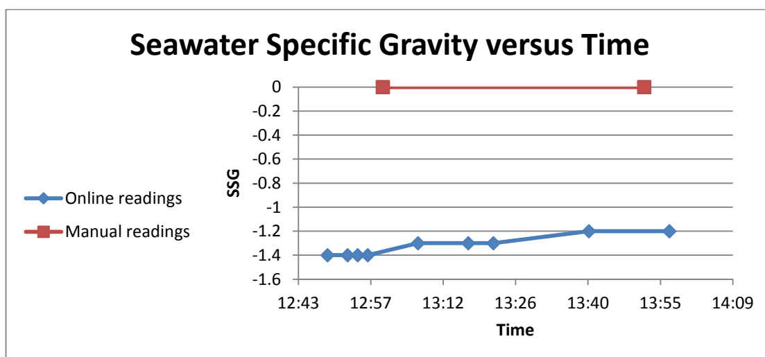
Figure 50 SSG change over time in Tuppurala, online and manual readings
