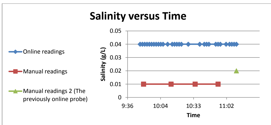
Figure 47 The salinity change over time in Pitkäjärvi, online and manual readings
